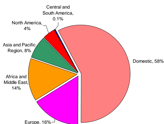
Chart 3.2: Regional distribution of scheduled passenger trips originating in Nigeria
