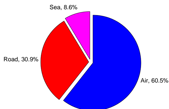
Chart 3.6: Foreign visitor arrivals by mode of transport
