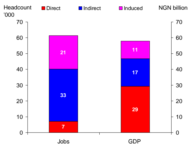
Chart 3.3: Nigerian jobs and output supported by airlines
