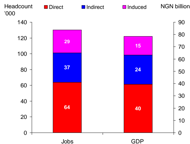
Chart 3.7: Travel and tourism's contribution to Nigerian GDP and Employment
