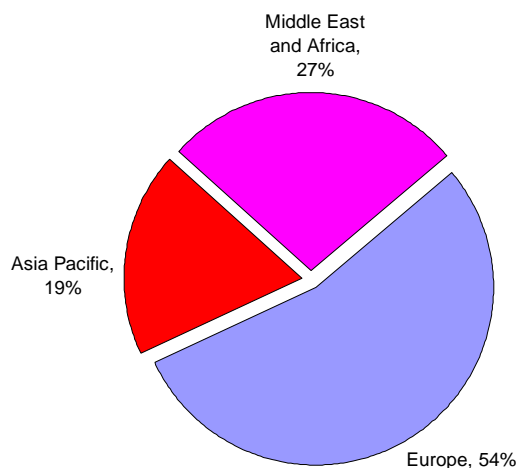
Chart 3.9: Regional distribution of Nigerian air freight (tonnes)
