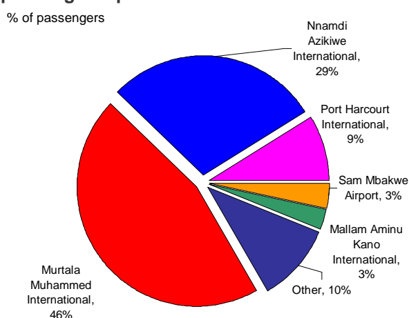
Chart 3.4: Regional distribution of Nigerian passenger trips
