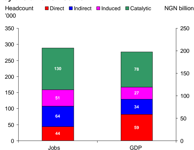
Chart 3.1: Nigerian Jobs and Output supported by the aviation sector
