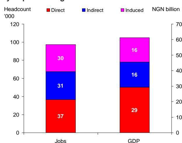
Chart 3.5: Nigerian jobs and output supported by airports and ground-based services
