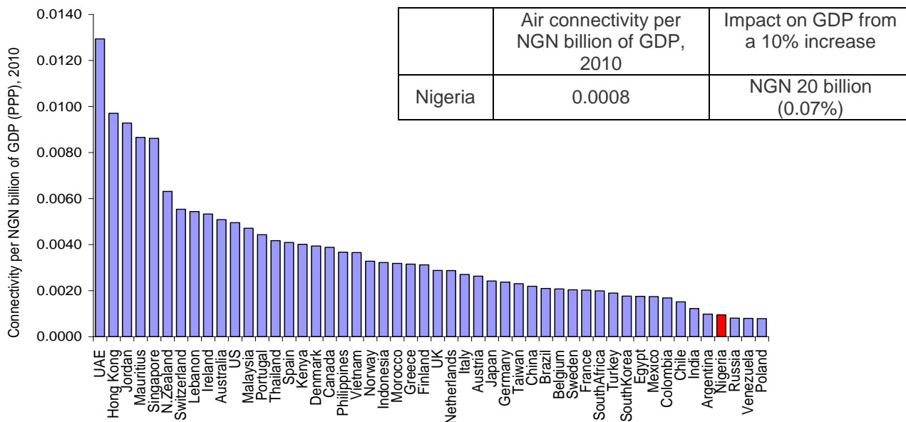
Chart 2.3: Air connectivity by country, 2010
